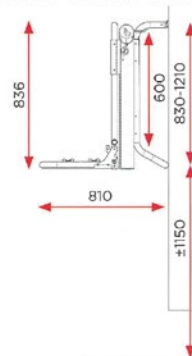
BIKE LIFT SHORT BIKE LIFT SHORT RAIL
