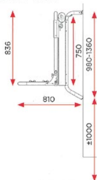
BIKE LIFT STANDARD BIKE LIFT RAIL
